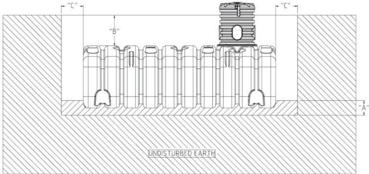
Figure 1: Site Excavation
