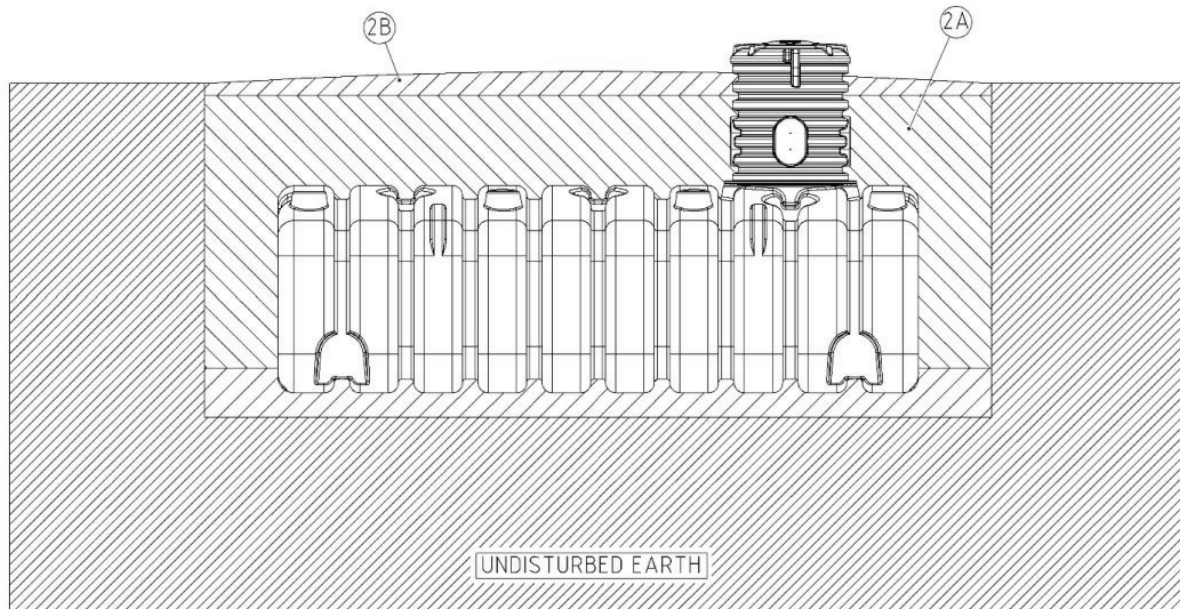
Figure 2: Site Backfilling
